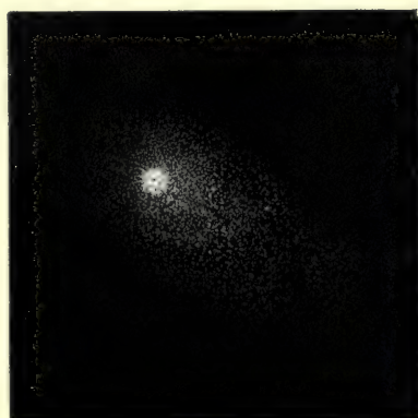
July 8.
